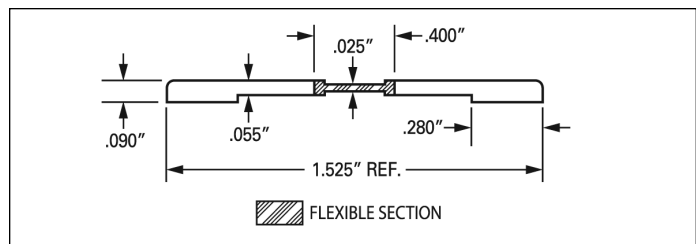
J-574 1.5" DR Flat
