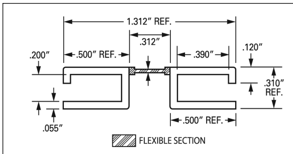
J-1191 .188" DR Channel
