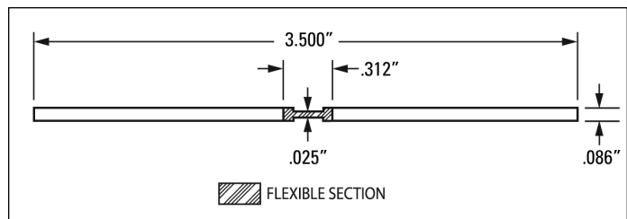
J-1197 3.5" PETG Flat J-1197 3.5" DR Flat
