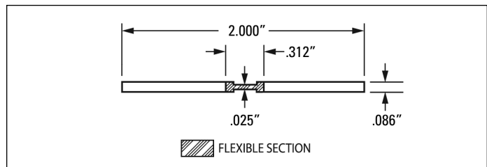
J-1196 2" PETG Flat J-1196 2" DR Flat
