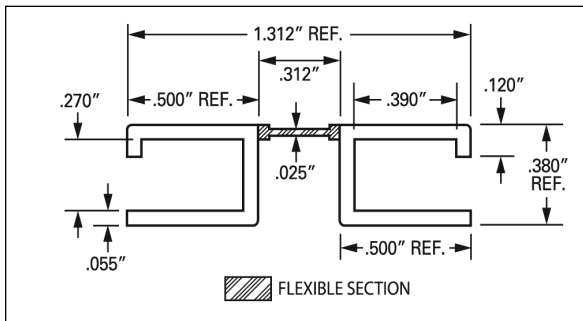
J-602 .25" DR Channel
