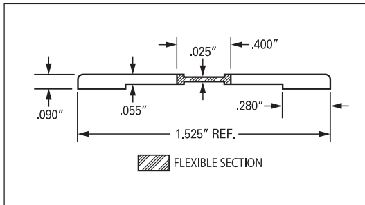
J-574 FLAT HINGE
