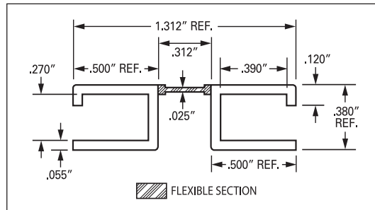
J-602 1/4" CHANNEL HINGE
