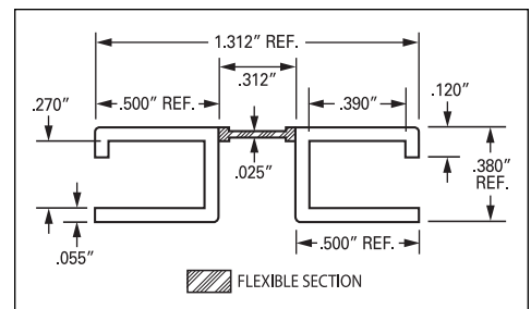
J-602 1/4" CHANNEL HINGE
