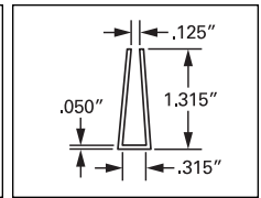
1 5/16" Channel PART NO. 3562
