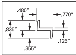
1/2" Z-Bar PART NO. J-1160
