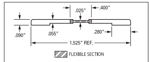
J-574 FLAT HINGE
