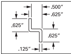
5/8" Z-Bar PART NO. 3845
