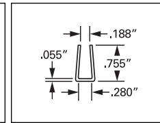
3/4" Channel PART NO. 4304
