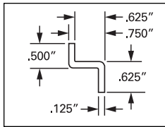
3/4" Z-Bar PART NO. 3872
