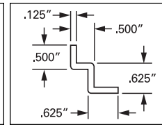
W-Bar PART NO. J-221
